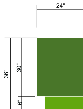
CORNER DETAIL (4) REQUIRED
