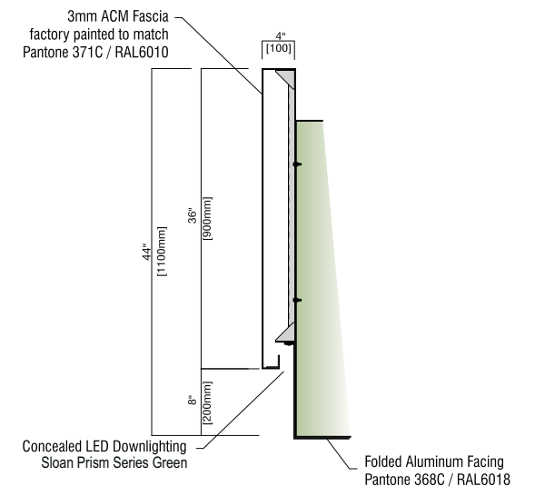
SECTION THRU ACCENT BAND
